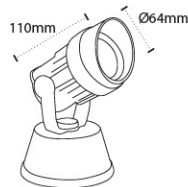
AL 5100 Cap W/L- 7W Color Temperature : 3000K, 6000K Material: Die-casting Aluminium, Metalised Reflector with Toughened Glass Body Color: Graphite Gray
