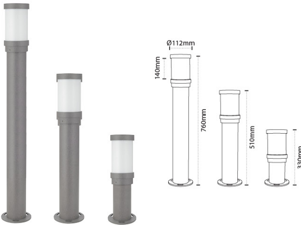
AL 2320-12W Colour Temperature : 3000K, 6000K Material : Die-casting Aluminium with PC Diffuser Body Color: Graphite Gray
