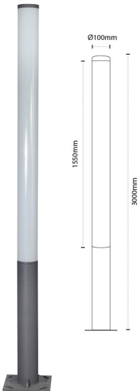
AL 3005 - 60W Colour Temperature : 3000K, 6000K Material : Galvanised MS Pole with PC Diffuser Body Color: Graphite Gray
