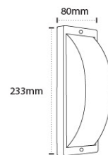
AL 1034 - 8W Color Temperature : 3000K, 6000K Material: Die-casting Aluminium with PC Diffuser Body Color: Graphite Gray
