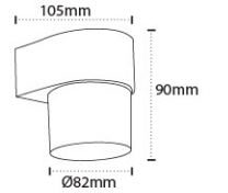
AL 1404 - 1x6W Color Temperature : 3000K, 6000K Material: Die-casting Aluminium with PC Diffuser Body Color: Graphite Gray
