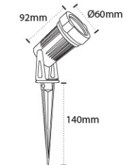
AL 4095 Spike LED: 5W Holder: GU-10, MR-16 Color Temperature : 3000K, 6000K Material: Die-casting Aluminium, Metalised Reflector with Toughened Glass Body Color: Black
