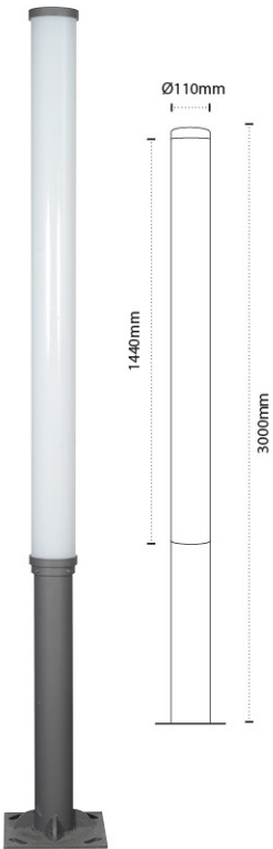
AL 2340 - 60W Colour Temperature : 3000K, 6000K Material : Galvanised MS Pole with PC Diffuser Body Color: Graphite Gray
