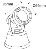
AL 5100 W/L- 7W Color Temperature : 3000K, 6000K Material: Die-casting Aluminium, Metalised Reflector with Toughened Glass Body Color: Graphite Gray
