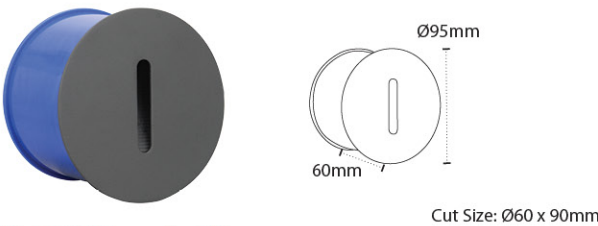
AL 8401 Round - 3W Color Temperature : 3000K, 6000K Material: Die-casting Aluminium, Toughened Glass with ABS Recess Box Body Color: Graphite Gray
