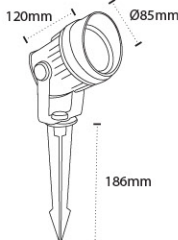
AL 5100 Cap- 12W Color Temperature : 3000K, 6000K Material: Die-casting Aluminium, Metalised Reflector, Toughened Glass with ABS Spike Body Color: Graphite Gray
