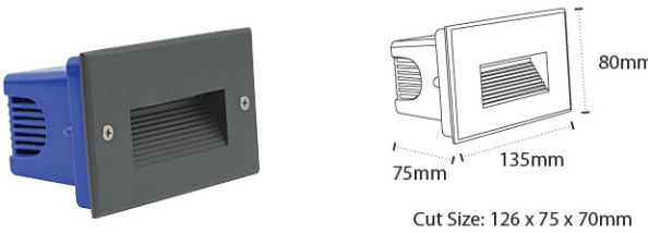
AL 9306 - 6W Color Temperature : 3000K, 6000K Material: Die-casting Aluminium, PC Diffuser with ABS Recess Box Body Color: Graphite Gray
