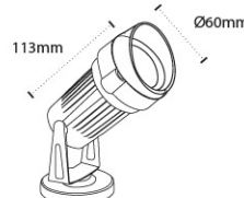
AL 4095 Cap W/L LED: 5W Holder: GU-10, MR-16 Color Temperature : 3000K, 6000K Material: Die-casting Aluminium, Metalised Reflector with Toughened Glass Body Color: Black
