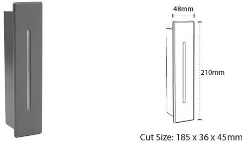
AL 9081 - 3W Color Temperature : 3000K, 6000K Material: Die-casting Aluminium, Toughened Glass with Metal Recess Box Body Color: Graphite Gray
