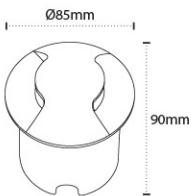
Cut Size: Ø75 x 70 mm AL 4050 - 2x1W Color Temperature : 3000K, 6000K Material: Die-casting Aluminium, PC Diffuer with ABS Recess Box Body Color: Graphite Gray
