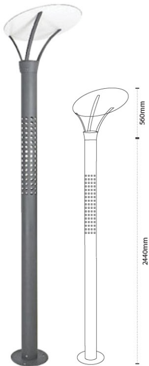
AL 777 40W + 60W Diffuser Colour Temperature : 3000K, 6000K Material : Galvanised MS, Aluminium Extruded Pole with PC Diffuser Body Color: Graphite Gray
