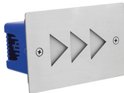
AL 3906-C - 4W Color Temperature : 3000K, 6000K Material: Die-casting Aluminium, S.S. 304 Grade Laser cut Plate, PC Diffuser with ABS Recess Box Body Color: Steel Finish
