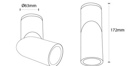
AL 882 - 5W Color Temperature : 3000K, 6000K Material: Die-casting Aluminium, Metalised Reflector with Toughened Glass Body Color: Graphite Gray
