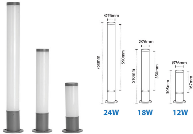
AL 3005 Colour Temperature : 3000K, 6000K Material : Die-casting Aluminium with PC Diffuser Body Color: Graphite Gray
