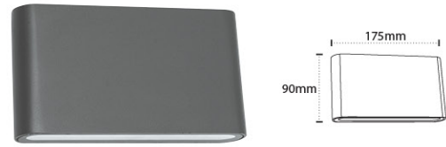
AL 234 - 2x8W Color Temperature : 3000K, 6000K Material: Die-casting Aluminium with Toughened Glass Body Color: Graphite Gray
