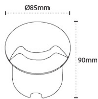
Cut Size: Ø75 x 70 mm AL 4050 - 1x1W Color Temperature : 3000K, 6000K Material: Die-casting Aluminium, PC Diffuer with ABS Recess Box Body Color: Graphite Gray
