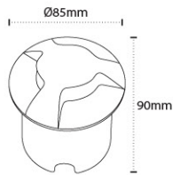
Cut Size: Ø75 x 70 mm AL 4050 - 3x1W Color Temperature : 3000K, 6000K Material: Die-casting Aluminium, PC Diffuer with ABS Recess Box Body Color: Graphite Gray
