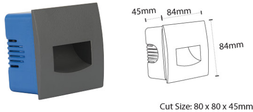
AL 33 - 3W Color Temperature : 3000K, 6000K Material: Die-casting Aluminium, PC Diffuser with ABS Recess Box Body Color: Graphite Gray
