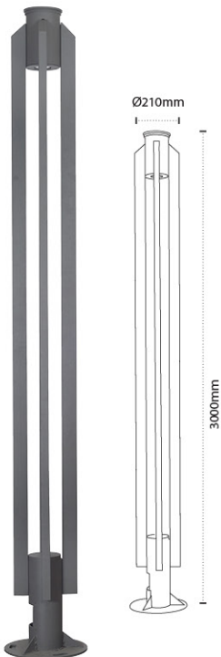
AL 8899 - 36W Colour Temperature : 3000K, 6000K Material : Galvanised MS Pipe with Toughened Glass Body Color: Graphite Gray
