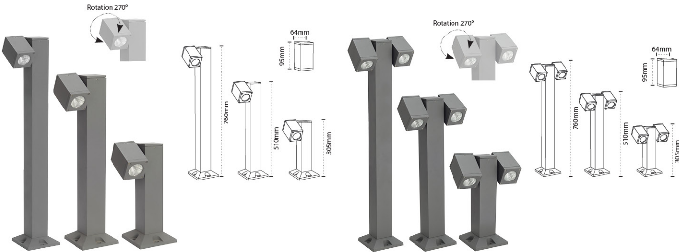
AL 6363 - 1x5W Colour Temperature : 3000K, 6000K Material : Die-casting Aluminium, Metalised Reflector with Toughened Glass Body Color: Graphite Gray
