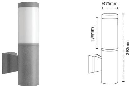
AL 6030 - 12W - Wall Light Colour Temperature : 3000K, 6000K Material : Die-casting Aluminium with PC Diffuser Body Color: Graphite Gray
