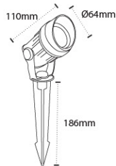
AL 5100 Cap- 7W Color Temperature : 3000K, 6000K Material: Die-casting Aluminium, Metalised Reflector, Toughened Glass with ABS Spike Body Color: Graphite Gray
