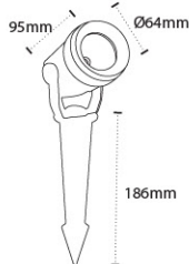
AL 5100 - 7W Color Temperature : 3000K, 6000K Material: Die-casting Aluminium, Metalised Reflector, Toughened Glass with ABS Spike Body Color: Graphite Gray
