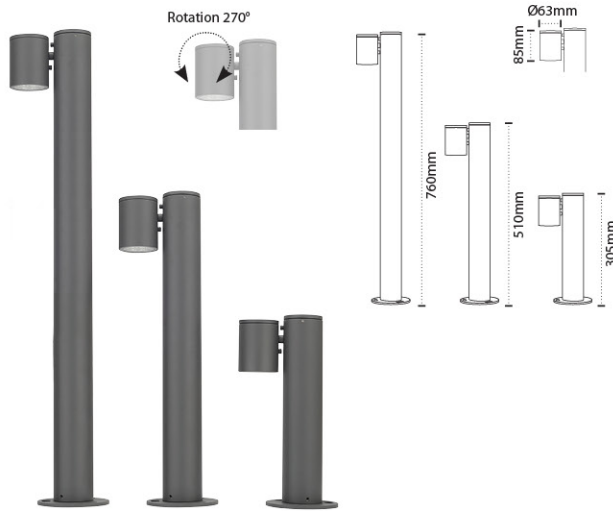
AL 8800 - 1x5W Colour Temperature : 3000K, 6000K Material : Die-casting Aluminium, Metalised Reflector with Toughened Glass Body Color: Graphite Gray
