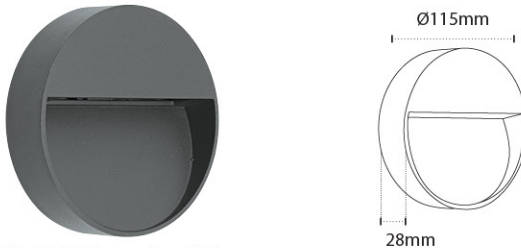
AL 990 Round - 4W Color Temperature : 3000K, 6000K Material: Die-casting Aluminium with Clear PC Body Color: Graphite Gray
