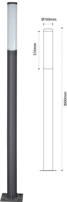
AL 6003 - 36W Colour Temperature : 3000K, 6000K Material : Galvanised MS Pole with PC Diffuser Body Color: Graphite Gray
