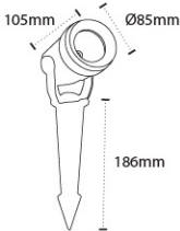
AL 5100 - 12W Color Temperature : 3000K, 6000K Material: Die-casting Aluminium, Metalised Reflector, Toughened Glass with ABS Spike Body Color: Graphite Gray
