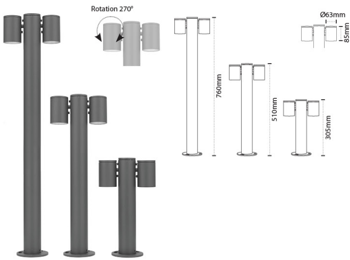
AL 8800 - 2x5W Colour Temperature : 3000K, 6000K Material : Die-casting Aluminium, Metalised Reflector with Toughened Glass Body Color: Graphite Gray
