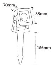
AL 4040- 7W Color Temperature : 3000K, 6000K Material: Die-casting Aluminium, Metalised Reflector, Toughened Glass with ABS Spike Body Color: Graphite Gray
