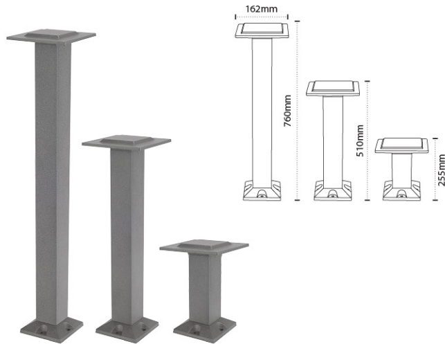
AL 7070 - 12W Colour Temperature : 3000K, 6000K Material : Die-casting Aluminium with PC Diffuser Body Color: Graphite Gray
