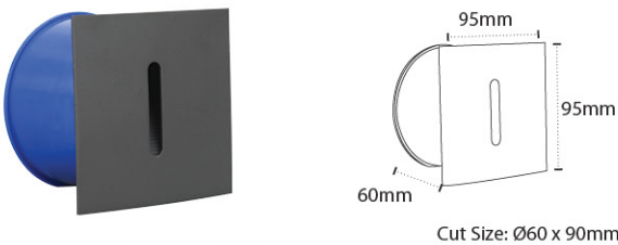
AL 8401 Square - 3W Color Temperature : 3000K, 6000K Material: Die-casting Aluminium, Toughened Glass with ABS Recess Box Body Color: Graphite Gray
