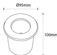
Cut Size: Ø85 x 93 mm AL 5050 - 7W Color Temperature : 3000K, 6000K Material: Die-casting Aluminium, 302 Grade SS Plate, Toughened Glass with ABS Recess Box Body Color: Steel Finish
