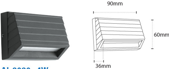
AL 8080 - 4W Color Temperature : 3000K, 6000K Material: Die-casting Aluminium with PC Diffuser Body Color: Graphite Gray
