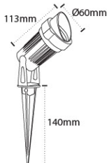
AL 4095 Cap Spike LED: 5W Holder: GU-10, MR-16 Color Temperature : 3000K, 6000K Material: Die-casting Aluminium, Metalised Reflector with Toughened Glass Body Color: Black
