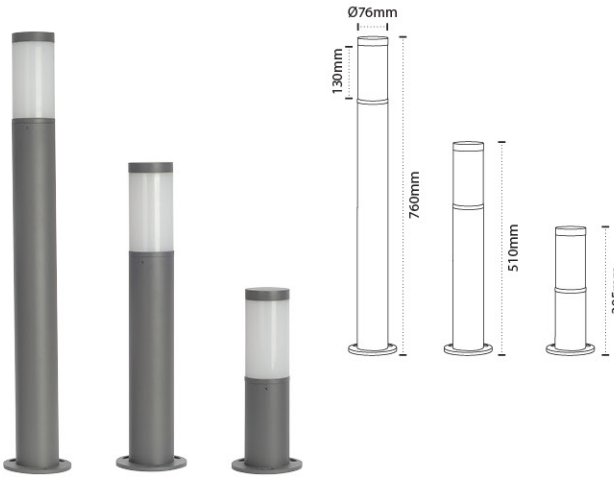
AL 6003 - 12W Colour Temperature : 3000K, 6000K Material : Die-casting Aluminium with PC Diffuser Body Color: Graphite Gray
