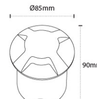
Cut Size: Ø75 x 70 mm AL 4050 - 4x1W Color Temperature : 3000K, 6000K Material: Die-casting Aluminium, PC Diffuer with ABS Recess Box Body Color: Graphite Gray
