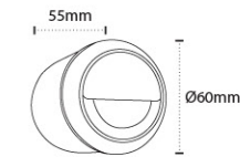
AL 26 A - 3W Color Temperature : 3000K, 6000K Material: Die-casting Aluminium, PC Diffuser with metal recess box Body Color: White
