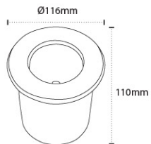
Cut Size: Ø106 x 105 mm AL 5050 - 12W Color Temperature : 3000K, 6000K Material: Die-casting Aluminium, 302 Grade SS Plate, Toughened Glass with ABS Recess Box Body Color: Steel Finish
