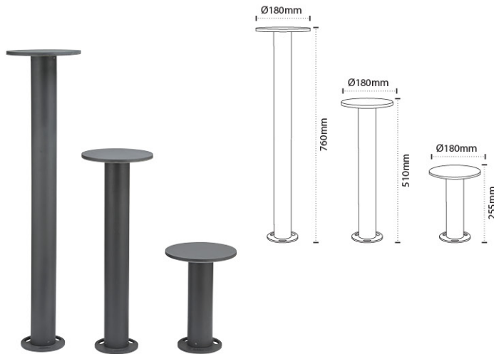
AL 7080 - 12W Colour Temperature : 3000K, 6000K Material : Die-casting Aluminium with PC Diffuser Body Color: Graphite Gray
