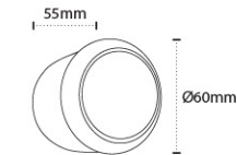
AL 26 B - 3W Color Temperature : 3000K, 6000K Material: Die-casting Aluminium, PC Diffuser with metal recess box Body Color: White
