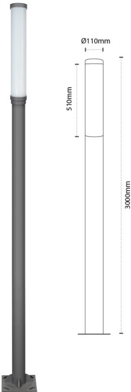
AL 2320 - 36W Colour Temperature : 3000K, 6000K Material : Galvanised MS Pole with PC Diffuser Body Color: Graphite Gray
