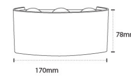
AL 642 - 6x3W Color Temperature : 3000K, 6000K Material: Die-casting Aluminium with Acrylic Lens Body Color: Graphite Gray
